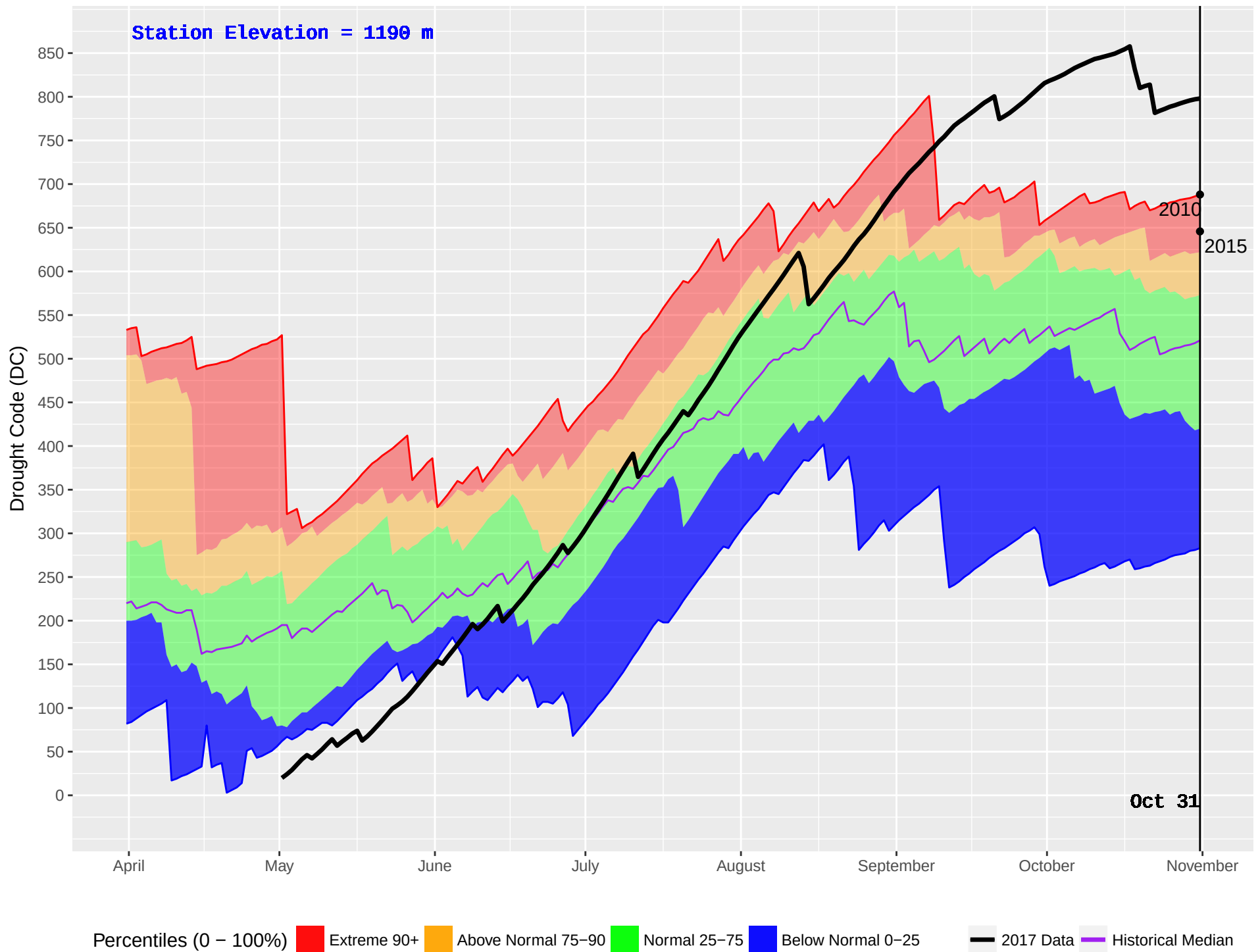
EMILY CREEK (425) : Historical (2002–2016) and Current (2017) Noon Drought Code (DC)
